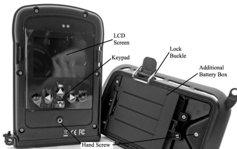
Figure 1.3: Back View
