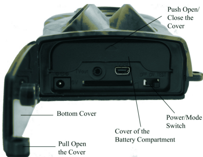
Figure 1.2: Bottom View-1
