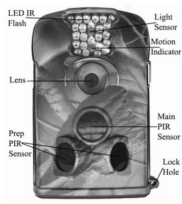
Figure 1.1: Front View
